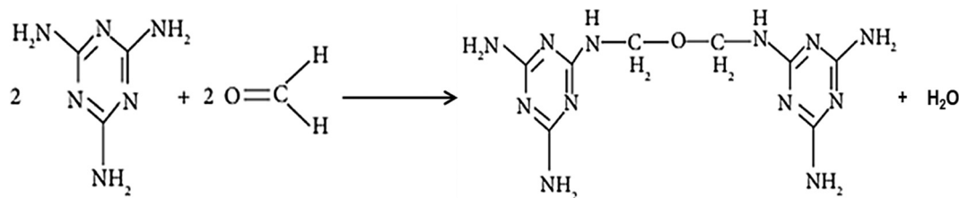
Fig. 3 Melamine-formaldehyde aerogels synthesized via a polycondensation reaction, enabling tunable density. Reproduced from ref. 44 with permission from Elsevier, copyright 2017.
