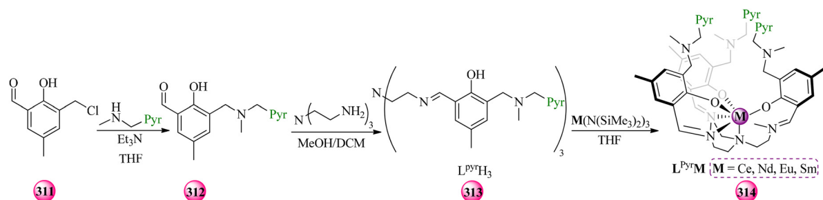
Fig. 86 Synthesis of pyrene-tagged lanthanide complexes containing heptadentate ligand L^{PyT}H_3 . Reproduced with permission from ref. 95 copyright 2017, Royal Society of Chemistry.
