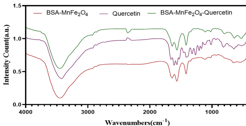
Fig. 3 FT-IR analysis of synthesized MnFe₂O₄-BSA-quercetin nanoparticles.
