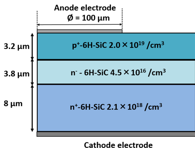
Fig. 8 Schematic representation of the simulated 6H-SiC p-n diode. 52
