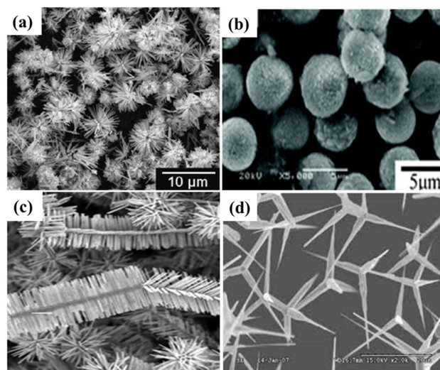
Fig. 3 Various 3D ZnO morphologies (a) ZnO NFs [Reprinted with permission from ref. 28 Copyright 2008, Elsevier] (b) ZnO hollow microspheres [Reprinted with permission from ref. 32 Copyright 2013, Royal society of chemistry] (c) ZnO hierarchical nanostructures [Reprinted with permission from ref. 33 Copyright 2002, American Chemical Society] (d) ZnO TPs nanostructures. 20
