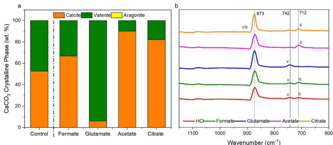
Fig. 13 (a) Refined Q-PXRD data of the PCC produced showing the polymorphs of CaCO 3 , vaterite, calcite, or aragonite, present in the samples; (b) FTIR spectral data of the carbonates produced showing characteristic CO 3 2- out-of-plane vibrational bending near 873 cm -1 , with vaterite characteristic peaks at 742 cm -1 and calcite in-the-plane bending at 712 cm -1 . 81–83 Table S2† shows the Rietveld refinement data and Fig. S6† shows the raw PXRD spectral data.
