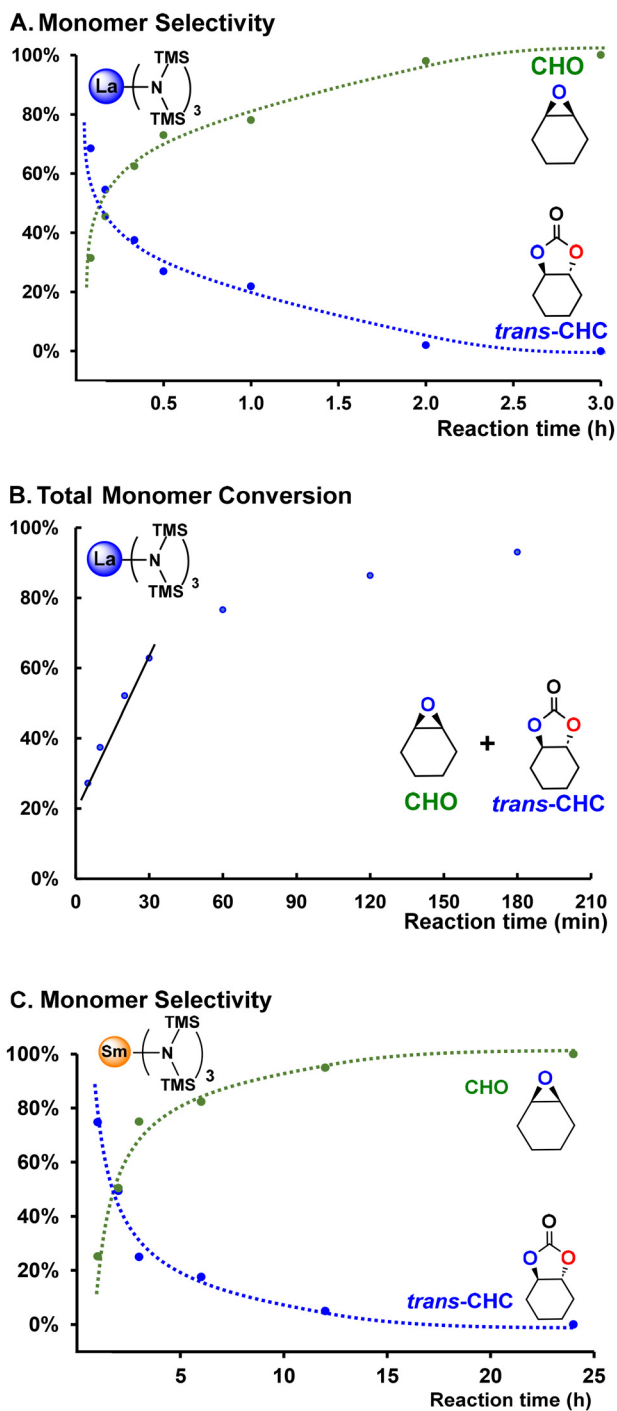
Fig. 1 A. Kinetic profile of PCHC depolymerization in a closed reaction system using \text{La}^{\text{NTMS}} under the conditions of Table 1. B. Total monomer conversion ( \text{trans-CHC} + \text{CHO} ) versus reaction time. C. Kinetic profile of PCHC depolymerization in a closed reaction system using \text{Sm}^{\text{NTMS}} .
