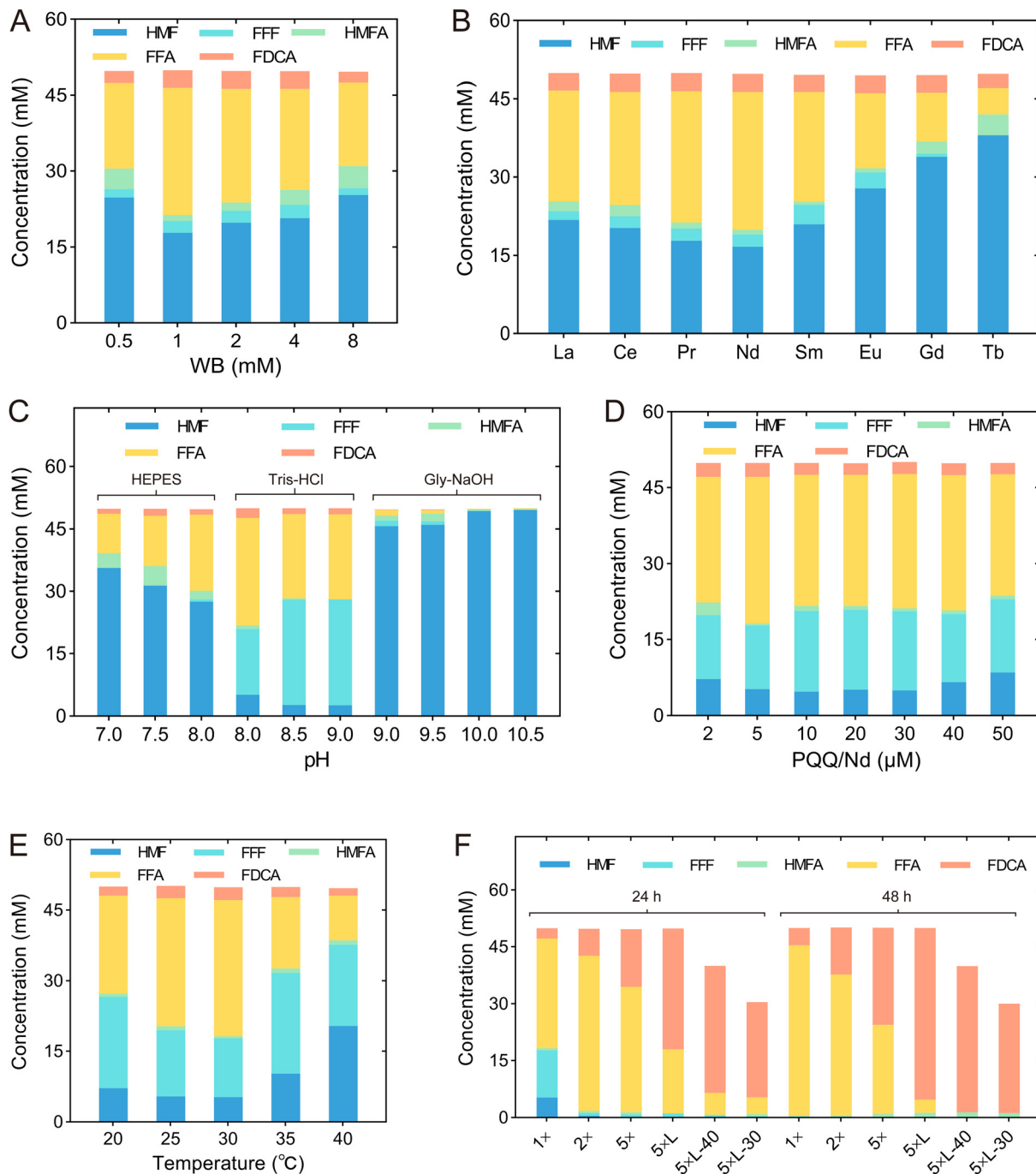
Fig. 6 Optimization of reaction conditions, including WB concentration (A), type of rare Earth element (B), pH (C), concentrations of PQQ and rare Earth elements (D), temperature (E), cell concentration and form of biocatalysts (F). 1x, whole cells with OD 600 of 10 used in the reaction; 2x, whole cells with OD 600 of 20 used in the reaction; 5x, whole cells with OD 600 of 50 used in the reaction; 5 × L, cell lysates with OD 600 of 50 used in the reaction; 5 × L-40, cell lysates with OD 600 of 50 used in the reaction with the 40 mM HMF; 5 × L-30, cell lysates with OD 600 of 50 used in the reaction with the 30 mM HMF.
