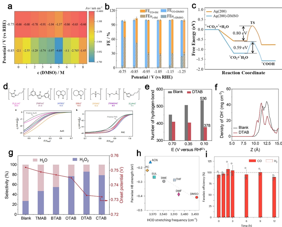
Fig. 13 (a) Heatmaps of CO partial current density at -0.75 V and -0.85 V in KCl–DMSO- x electrolyte. FE in (b) \text{CO}_2 -saturated with and without DMSO additive. 167 Copyright 2023, Wiley-VCH. (c) Energy barriers of transitional state formation for ^*\text{CO}_2 to ^*\text{COOH} conversion with and without DMSO additive. 167 Copyright 2023, Wiley-VCH. (d) The ORR activity on ionic-liquid-modified Au/C and Pt/C measured in \text{O}_2 -saturated 0.1 M \text{HClO}_4 . 36 Copyright 2021, Nature Publishing Groups. (e) Number of hydrogen bonds in KOH and DTAB-modified KOH electrolyte at 0.10 V_{\text{RHE}} . (f) Radial density distribution of \text{OH}^- in KOH and DTAB-modified KOH electrolyte at 0.10 V_{\text{RHE}} . (g) The \text{H}_2\text{O}_2 selectivity and onset potential at 0.3 V_{\text{RHE}} in KOH electrolytes. 166 Copyright 2024, American Chemical Society. (h) The pairwise HB strength from DFT calculations and the HOD stretching frequency extracted for 1 M water in different solvents. (i) Product distribution analysis for DMSO solution using a zinc electrode at -10 \text{mA cm}^{-2} over 12 h electrolysis. 175 Copyright 2024, Nature Publishing Groups.
