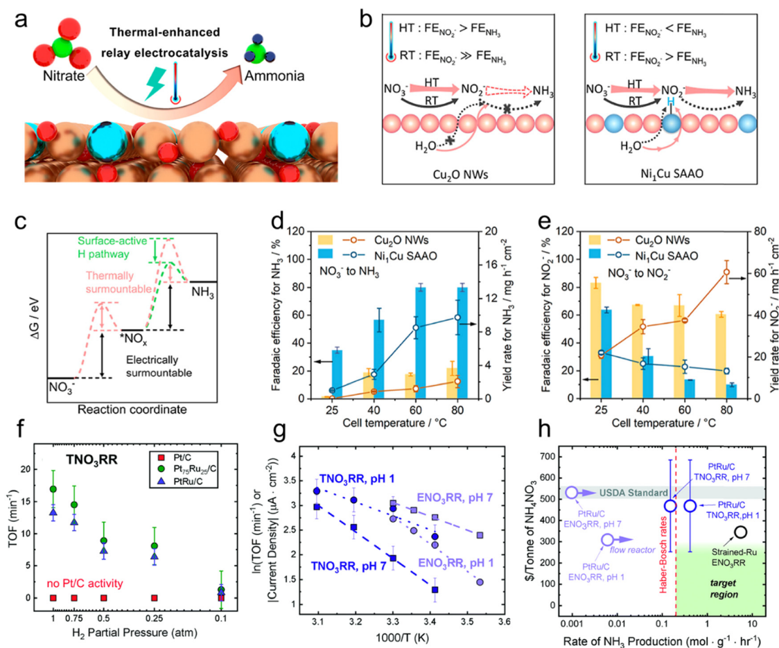
Fig. 10 (a) Thermal-assisted electrocatalysis \text{NO}_3\text{RRs} on \text{Ni}_1\text{Cu} SAAO NWs. (b) Mechanism diagram of the \text{NO}_3\text{RR} at different temperatures using \text{Ni}_1\text{Cu} SAAO and \text{Cu}_2\text{O} NWs. HT, RT, and FE are high temperature, room temperature, and faradaic efficiency, respectively. (c) The energy barrier overcome by thermally boosted electrocatalysis and surface-active hydrogen during \text{NO}_3^- reduction on \text{Ni}_1\text{Cu} SAAO. Faradaic efficiency and yield rate for (d) \text{NH}_3 and (e) \text{NO}_2^- production at different temperatures using \text{Ni}_1\text{Cu} SAAO and \text{Cu}_2\text{O} NWs at 0.1 V vs. RHE. Reproduced with permission. 125 Copyright 2024, American Chemical Society. (f) The activity of various catalysts in thermocatalytic \text{NO}_3\text{RR} at different \text{H}_2 partial pressures in pH 7 solution with 0.1 M \text{NaNO}_3 . (g) Arrhenius plots of PtRu/C for thermocatalytic and electrocatalytic \text{NO}_3\text{RRs} . (h) The cost per tonne of \text{NH}_4\text{NO}_3 in thermocatalytic and electrocatalytic \text{NO}_3\text{RRs} vs. \text{NH}_3 yield rate. Reproduced with permission. 126 Copyright 2021, Royal Society of Chemistry.
