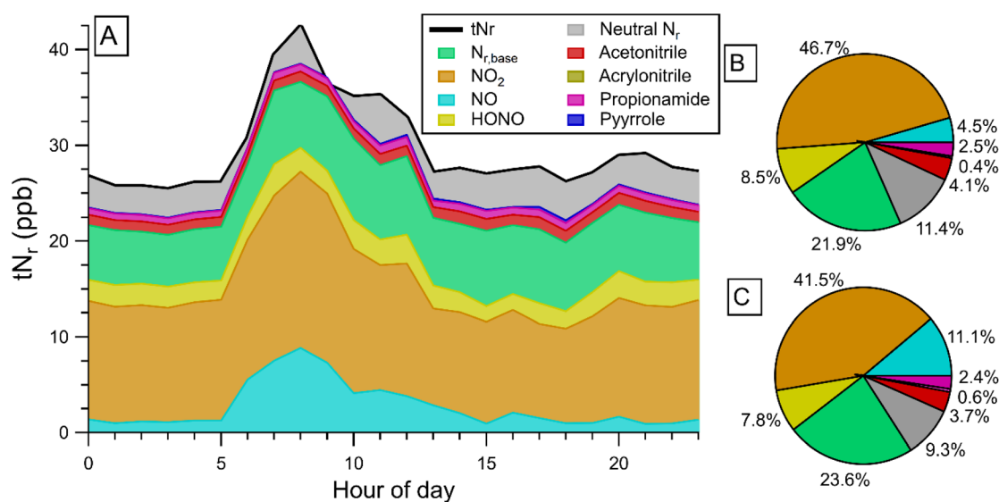
Fig. 4 (A) Cumulative mean diurnal trends of quantified t\text{N}_r and sub-species along with calibrated N-containing ions thought to arise from neutral molecules detected by PTR-MS. Pie charts represent the average gaseous \text{N}_r budget (B) at night when operations ceased (10 pm to 6 am), and (C) during occupation for daytime cooking (9 am to 8 pm).
