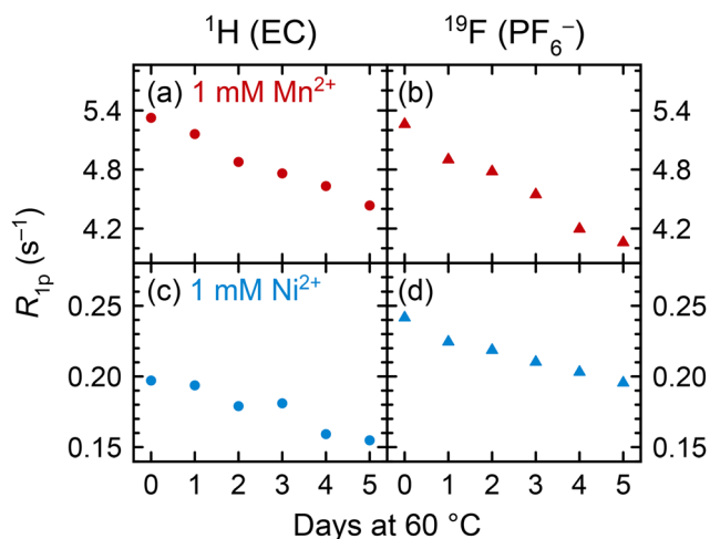
Fig. 4 (a) and (c) 1 H EC (circles) and (b) and (d) 19 F PF 6 − (triangles) longitudinal paramagnetic relaxation rates ( R_{1p} ) of Mn 2+ - or Ni 2+ -containing electrolyte solutions across five days of heating at 60 °C. Electrolyte solutions comprised 1 M LiPF 6 in 3 : 7 EC : EMC (v/v) with 1 mM Mn(TFSI) 2 (red) or Ni(TFSI) 2 (blue). Solutions were cooled to ambient temperature (~25 °C) before relaxation rates were measured.
