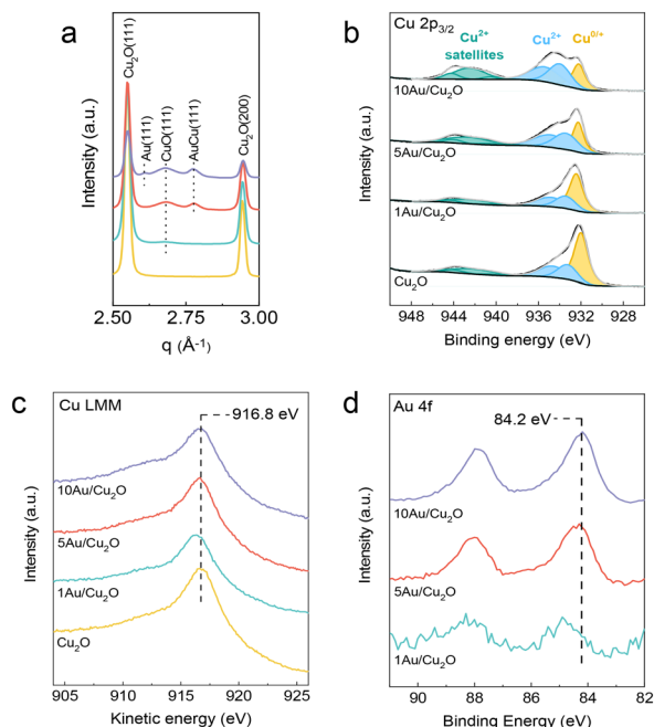
Fig. 2 (a) Synchrotron X-ray diffractograms of the as-prepared samples ( \lambda = 0.0165312 nm). (b) Cu 2p_{3/2} LMM and (d) Au 4f XPS spectra of the as-prepared samples.
