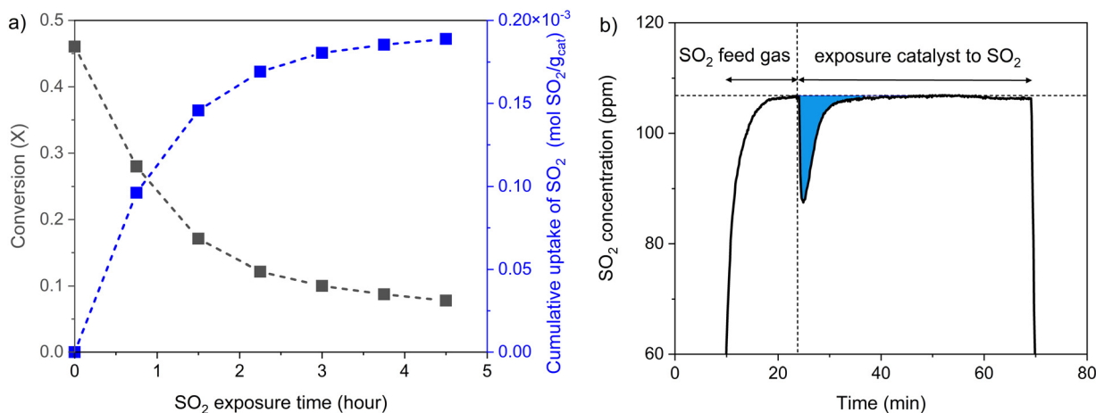
Fig. 1 a) Measured conversion and accumulated \text{SO}_2 uptake in six consecutive \text{SO}_2 exposure cycles at 200 °C after formation of the [(\text{NH}_3)_4\text{Cu}_2\text{O}_2]^{2+} complex. b) Measured \text{SO}_2 concentration during exposure to \text{SO}_2 . The blue area represents the uptake of \text{SO}_2 . Catalyst 3.2 wt% Cu-CHA, Si/Al ratio 6.7.
