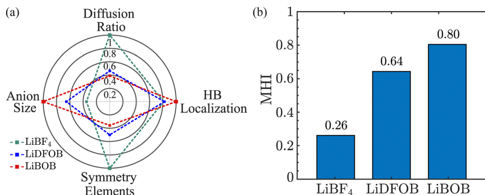
Fig. 11 (a) Radar plot comparing key molecular features: diffusion ratio, HB localization, anion size, and number of symmetry elements, and (b) bar chart of MHI for the \text{LiBF}_4 , LiDFOB, and LiBOB-based DEEs.
