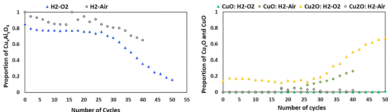
Fig. 6 Changes in the relative percentages of \text{Cu}_x\text{Al}_y\text{O}_4 (left) and \text{Cu}_2\text{O} –CuO phases (right) at the end of the oxidation reactions from fresh sample to up to 50 cycles for \text{H}_2\text{-O}_2 and \text{H}_2\text{-air} datasets.
