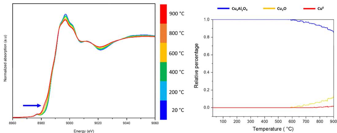
Fig. 1 Spectral evolution during ramp up for \text{H}_2\text{--O}_2 (left) and the corresponding concentration profile of the \text{Cu}_x\text{Al}_y\text{O}_z , \text{Cu}_2\text{O} and \text{Cu}^0 as a function of the temperature ramp under 2.5% \text{O}_2 .
