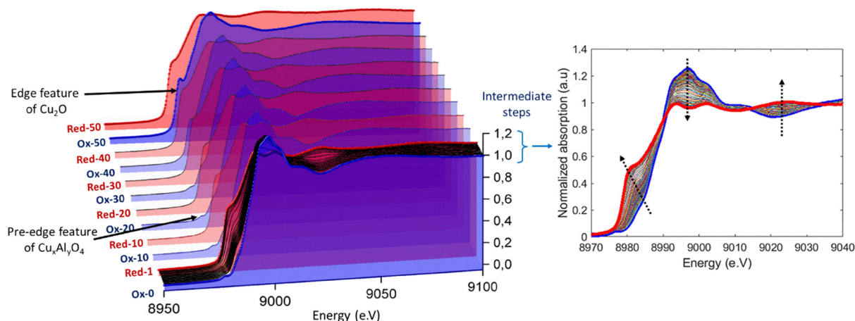
Fig. 2 Spectral change over 50 redox cycles represented for every 10 cycles for the 2.5% \text{H}_2\text{--}2.5\% \text{O}_2 sample.
