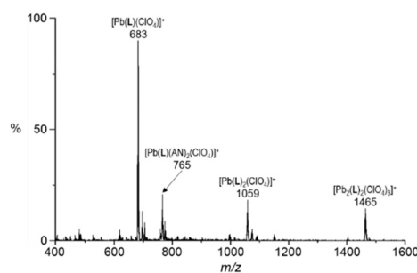
Fig. 4 ESI-mass spectrum of a mixture of L and \text{Pb}(\text{ClO}_4)_2 \cdot 3\text{H}_2\text{O} in \text{CH}_2\text{Cl}_2/\text{CH}_3\text{CN} (1:1, v/v).
