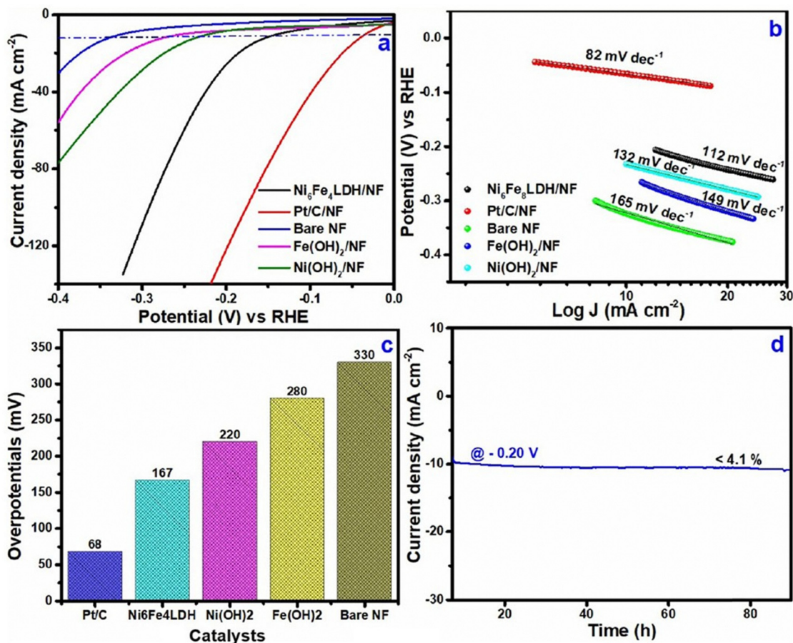
Fig. 6 HER (a) LSV curves (b) Tafel plot (c) overpotentials (at 10\text{ mA cm}^{-2} ) of \text{Ni}_6\text{Fe}_4\text{LDH/NF} , \text{Pt/C/NF} , \text{Ni(OH)}_2/\text{NF} , \text{Fe(OH)}_2/\text{NF} and bare NF (d) current density vs. time plot for \text{Ni}_6\text{Fe}_4\text{LDH/NF} (reproduced with permission from ref. 26 ©2024, The American Chemical Society).
