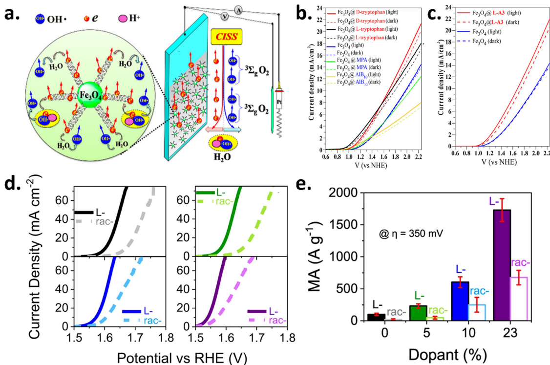
Fig. 6 Chiral functionalization of Fe 3 O 4 and Co 3 O 4 -based nanoparticles and enhancement of spin-selectivity for the OER. (a) Schematic of chiral-functionalized electrodes, where the C 1 S 2 S effect enhances the OER via triplet oxygen production. (b) Photocurrent and dark current densities for Fe 3 O 4 NPs linked to chiral (D- and L-tryptophan) and achiral (mercaptopyronic acid, azo isobutyric acid) molecules, compared to pure Fe 3 O 4 NPs. (c) Photocurrent density of Fe 3 O 4 NPs linked to chiral L-A3 versus pure Fe 3 O 4 NPs. (d) LSV plot showing undoped (black) and iron-doped Rac- (dashed) and L-cobalt oxide (solid) nanoparticle catalysts in Nafion, with doping levels of 5% (green), 10% (blue), and 23% (purple), measured in 1 M NaOH. (e) Mass activity (MA) comparison of Rac- (open symbols) and L-cobalt oxide (filled symbols) nanoparticle catalysts in Nafion. Figures are adopted from ref. 24 and 26 with permission from American Chemical Society © 2018 and Nature © 2023.
