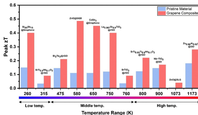
Fig. 9 Peak zT values of pristine materials and graphene composites: (1) \text{Bi}_{0.85}\text{Sb}_{0.15}/\text{graphene} , 114 (2) \text{SrTi}_{0.9}\text{Nb}_{0.1}\text{O}_3/\text{rGO} , 115 (3) \text{Bi}_2\text{Te}_3/\text{rGO} , 116 (4) \text{ZnO}/\text{GQD} , 12 (5) \text{CoSb}_3/\text{graphene} , 117 (6) \text{La}_{0.067}\text{Sr}_{0.9}\text{TiO}_3/\text{rGO} , 113 (7) \text{SrTiO}_3/\text{rGO} , 52 (8) \text{Sr}_{0.93}\text{Ti}_{0.90}\text{Nb}_{0.10}\text{O}_3/\text{rGO} , 118 (9) \text{Nb}-\text{TiO}_2/\text{GO} , 55 (10) \text{ZnO}/\text{SLG} , 119 and (11) \text{Zn}_{0.98}\text{Al}_{0.02}\text{O}/\text{GO} . 51
