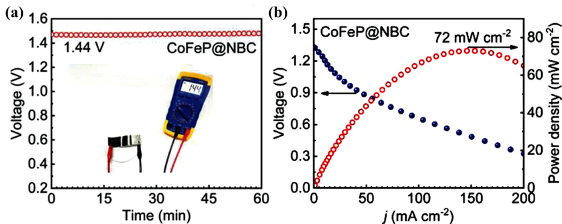
Fig. 12 (a) Plot illustrating the OCV of a quasi-solid-state ZAB based on CoFeP@NBC. (b) Discharge polarization and corresponding power densities curves of the quasi-solid-state ZAB. Inset in (a) is the digital image of the ZAB. Reproduced with permission from ref. 126. Copyright 2024 Wiley.
