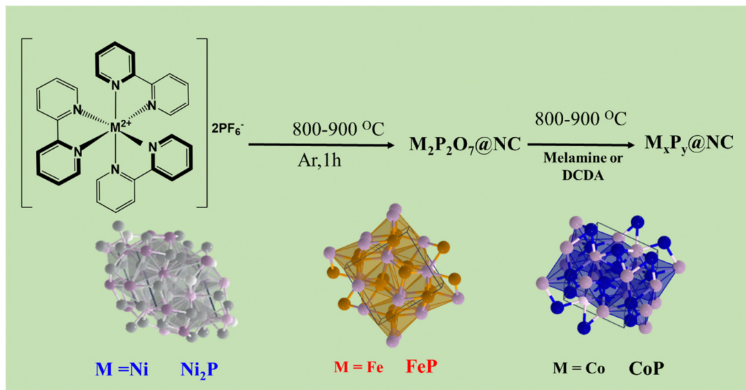
Fig. 4 Universal method for the synthesis of heteroatom-doped graphitic carbon encapsulated TMPs using a metal polypyridyl complex as a single source precursor. Ni_2P@NC , FeP@NC , and CoP@NC are synthesized using the corresponding polypyridyl complexes.
