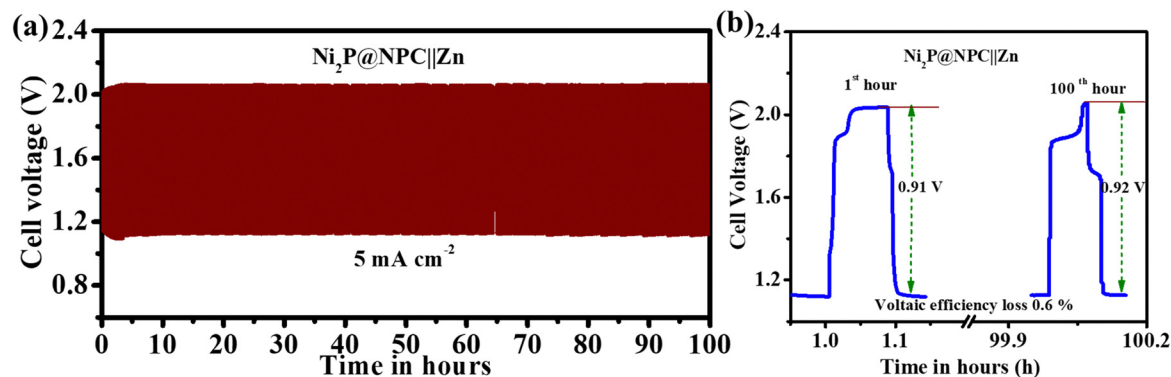
Fig. 11 (a) Galvanostatic charge–discharge cyclability of the Ni 2 P@NPC-based ZAB at 5 mA cm -2 . (b) Voltaic efficiency plots of Ni 2 P@NPC||Zn. Reproduced with permission from ref. 64. Copyright 2024 Wiley.
