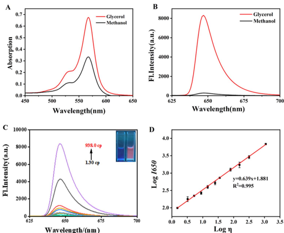
Fig. 2 (A) UV-vis spectrum of LTP-H (10 \mu\text{M} ) in MeOH and Gly. (B) FL spectra of LTP-H (10 \mu\text{M} ) in MeOH and Gly. (C) FL spectra of LTP-H (10 \mu\text{M} ) with variation of the solution viscosity (1.30–938.0 cp). (D) Linear correlation between \log I_{650} and \log \eta ; \lambda_{\text{ex}} = 570 nm, \lambda_{\text{em}} = 650 nm.
