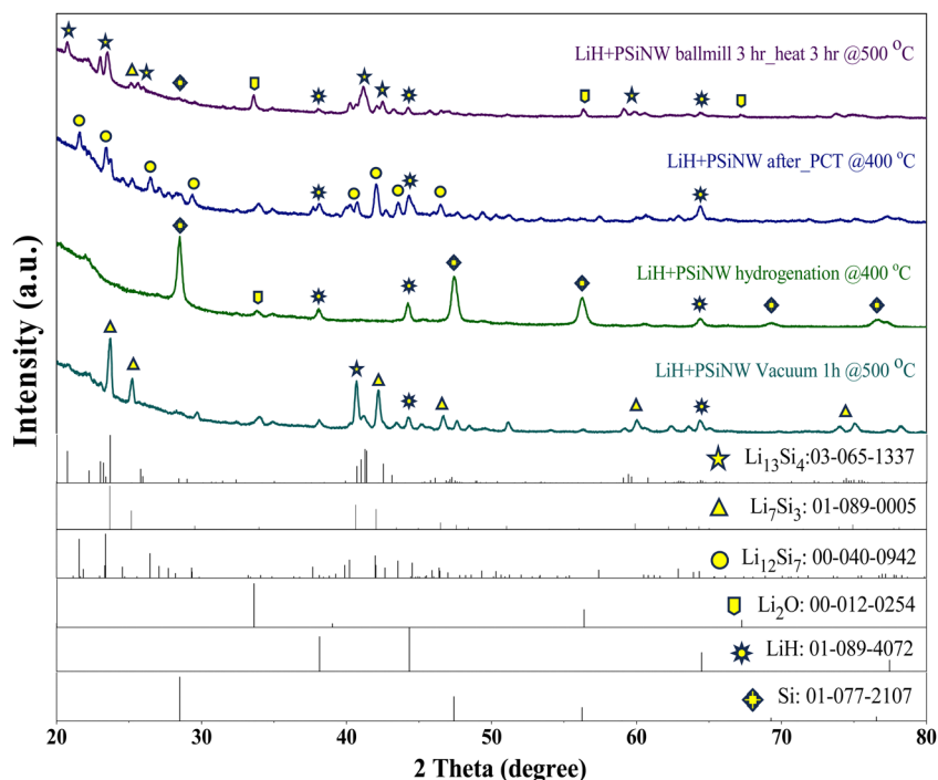
Fig. 4 XRD analytical technique of the LiH–PSiNW alloy at four different stages (peaks of coner phases are leveled): after ball milling followed by 3 hours of heat treatment at 500 °C for alloy formation, after the PCT cycle at the optimized temperature (400 °C), after hydrogenation at 400 °C, and followed by hydrogen desorption (500 °C for 1 hour) after PCT (400 °C).
