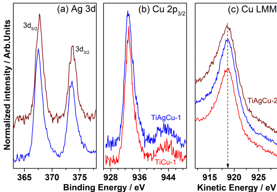
Fig. 5 XPS core level spectra recorded for (a) Ag 3d and (b) Cu 2p_{3/2} core levels, and (c) X-ray initiated Auger electron spectra recorded for Cu- L_3M_4M_45 transition for TiCu-1, TiAgCu-1 and TiAgCu-2 nanocomposites. Different colours were used for different compositions, namely, TiCu-1 (red), TiAgCu-1 (blue), and TiAgCu-2 (brown).
