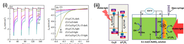
Fig. 8 (i) (a) Transient photocurrent response at a bias potential of -0.4 V (vs. Ag/AgCl) under visible light: [(1) \text{Cu}_2\text{O} ; (2) \text{Cu}_2\text{O}/\text{g-C}_3\text{N}_4-5 ; (3) \text{Cu}_2\text{O}/\text{g-C}_3\text{N}_4-10 ; (4) \text{Cu}_2\text{O}/\text{g-C}_3\text{N}_4-15 ; (5) \text{Cu}_2\text{O}/\text{g-C}_3\text{N}_4-20 ; (6) \text{g-C}_3\text{N}_4 ]. (b) Linear sweep voltammograms of \text{Cu}_2\text{O} , \text{g-C}_3\text{N}_4 and \text{Cu}_2\text{O}/\text{g-C}_3\text{N}_4-15 films in the dark and under visible light. (ii) Schematic pathway for photoelectron transfer and the photoelectrochemical process in \text{Cu}_2\text{O}/\text{g-C}_3\text{N}_4 film under visible light irradiation. Reprinted from ref. 151 with permission.
