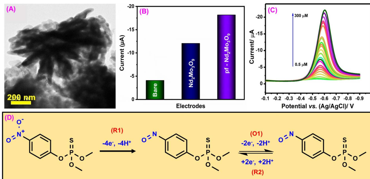
Fig. 2 (A) TEM image of pf- \text{Nd}_2\text{Mo}_3\text{O}_9 . (B) CV investigation of the bare GCE (green), \text{Nd}_2\text{Mo}_3\text{O}_9 (blue), and pf- \text{Nd}_2\text{Mo}_3\text{O}_9 (purple). (C) DPV signal of pf- \text{Nd}_2\text{Mo}_3\text{O}_9 for MPN detection. (D) Electrochemical detection mechanism of MPN 103 (modified). ((A and C) License number: 5542351439158).
