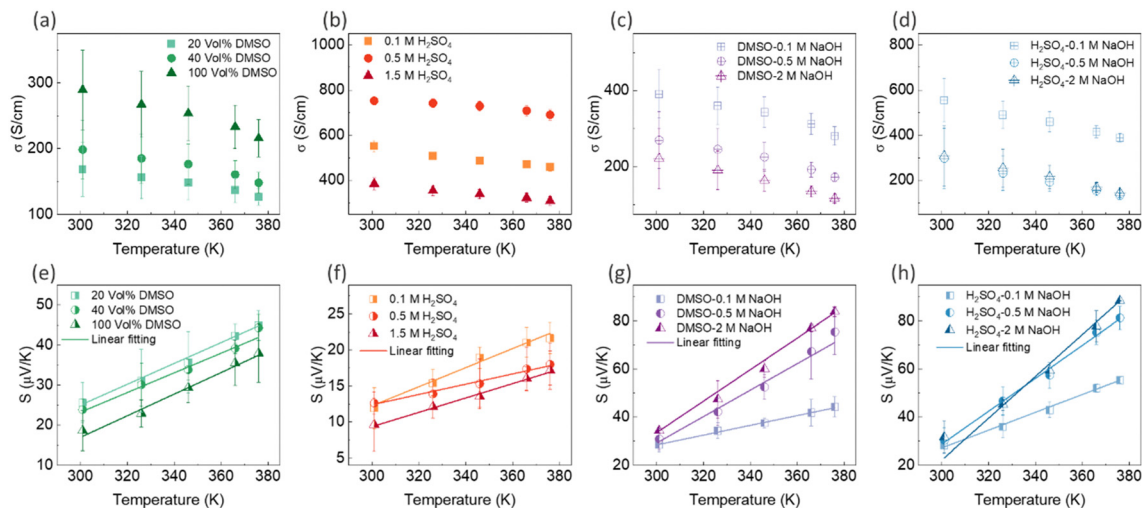
Fig. 8 The variation in electrical conductivity and Seebeck coefficient with temperature for PEDOT:PSS/40 wt% BST thin films after: single post-treatment with DMSO (a) and (e), H_2SO_4 (b) and (f), sequential post-treatment with DMSO–NaOH (c) and (g), and H_2SO_4 –NaOH (d) and (h). The dashed lines in (e)–(h) represent the linear fitting of eqn (7) to the experimental data. The error bars on the experimental data were calculated based on three repetitions of measurements on the samples.
