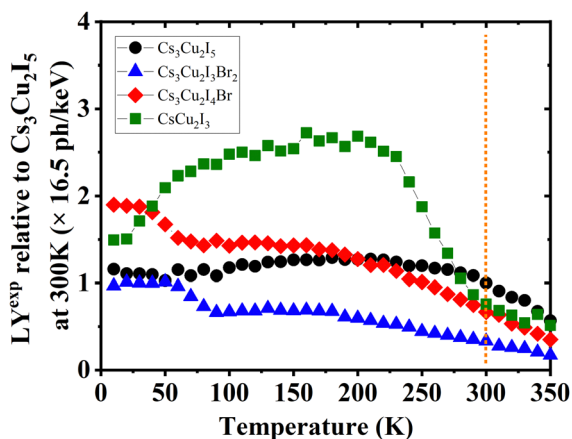
Fig. 6 Temperature-dependent experimental LY ( LY^{\text{exp}} ) spectra of Cs_3Cu_2I_5 , Cs_3Cu_2I_4Br , Cs_3Cu_2I_3Br_2 , and CsCu_2I_3 , normalised to the LY of Cs_3Cu_2I_5 at 300 K derived using integrated RL intensities. The vertical dashed line indicates where the value of LY^{\text{exp}} is taken using pulse height spectra at RT, see Fig. S13 (ESI†).
