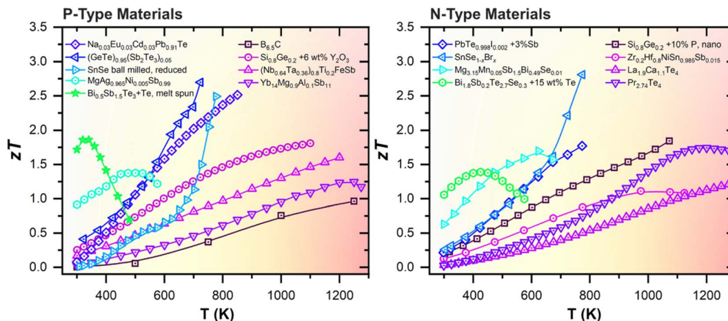
Fig. 2 Temperature-dependent figures-of-merit ( zT ) of state-of-the-art TE materials based on (Bi, Sb) 2 (Te, Se) 3 , 55,56 Mg 3 (Sb, Bi) 2 , 57 MgAgSb, 58 GeTe, 59 PbTe, 38,60 SnSe, 41,42 half Heusler alloys, 61,62 B 4 C, 63 Si 0.8 Ge 0.2 , 64,65 Yb 14 MgSb 11 , 66 La 3-x Te 4 , 67 and Pr 3-x Te 4 . 68
