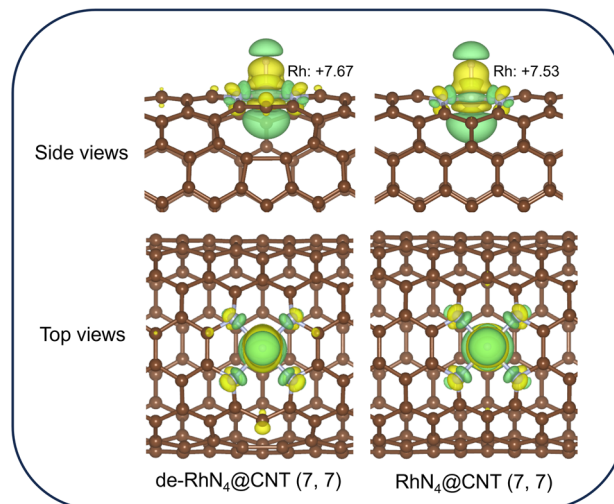
Fig. 8 Bader charge, and charge density difference for H atom adsorption on RhN 4 @CNTs (7,7) and de-RhN 4 @CNTs (7,7). The yellow region represents charge accumulation, and the cyan region represents charge depletion. The isosurface value is 0.002 e bohr -3 .
