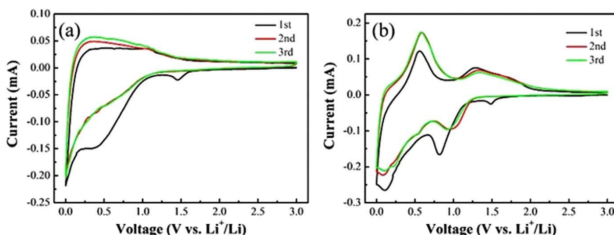
Figure 5: Cyclic voltammety plots for the first three cycles of (a) carbon fibre anodes and (b) a CFBA consisting of SnO 2 coated carbon fibres 25 . Reproduced from reference [25] with permission from Elsevier, copyright 2024.
