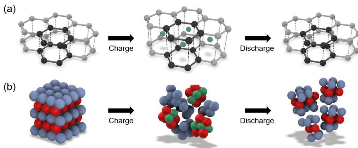
Figure 3: Illustration of the effect of charging and discharging in (a) graphite, an intercalation-type anode and (b) \text{SnO}_2 , a conversion-type anode. Green spheres are \text{Li}^+ ions, black/grey spheres are carbon, red spheres are \text{O}^{2-} ions, and blue spheres are \text{Sn}^{4+} ions/ \text{Sn} metal. In the case of the conversion-type anode, the illustration shows the material going from a pristine state prior to charging to a pulverised state after the first discharge.
