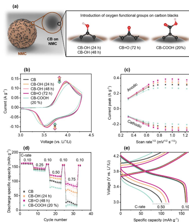
Fig. 2 Electrochemical tests for NMC622 cathodes fabricated using modified CBs. (a) Schematic of oxygen-containing functional groups on CB. (b) CV with a scan rate of 0.1\text{ mV s}^{-1} . (c) Anodic and cathodic current peaks at a scan rate of 0.1\text{--}1.5\text{ mV s}^{-1} versus the square root of the scan rate ( \text{mV}^{1/2}\text{ s}^{-1/2} ), a linear interval of 0.1\text{--}0.4\text{ mV s}^{-1} was fitted. (d) Rate performance of the NMC622 cathodes at 0.10, 0.25, 0.50, and 0.75 C-rates, error bars represent standard deviations. (e) GCD curves at 0.1 and 0.5 C-rates.
