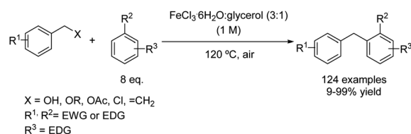
Scheme 6 \text{FeCl}_3/\text{glycerol} promoted synthesis of diaryllkanes.
