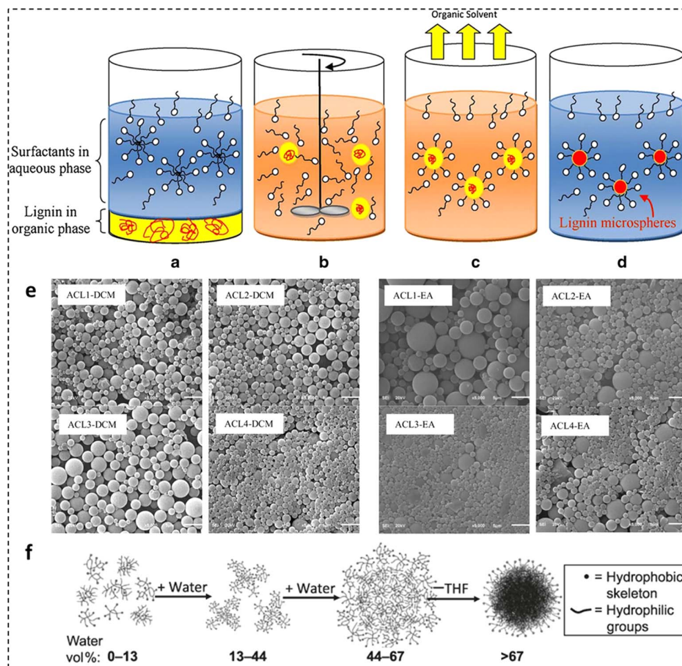
Fig. 3 Four steps of ESE: (a) addition of two phases with opposite polarities, (b) emulsification, (c) evaporation of the solvent phase, and (d) microparticle formation, (e) lignin microsphere SEM micrographs (reproduced from ref. 72 with permission from Wiley, copyright 2012), and (f) lignin microsphere formation employing solvent exchange (reproduced from (ref. 84) with permission from RSC, copyright 2014).
