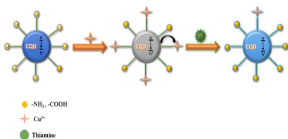
Fig. 10 Fluorescence quenching of CQDs by \text{Cu}^{2+} following the PET mechanism and the recovery of fluorescence after adding thiamine. 98
