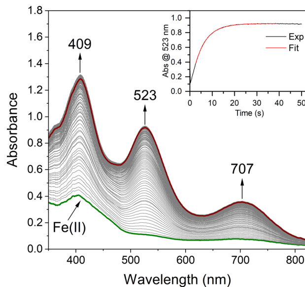
Fig. 1 Time-resolved spectral changes obtained upon mixing THF solutions of five-coordinate [\text{Fe}^{\text{II}}(\text{S}_2\text{Me}_2\text{N}_3(\text{Pr,Pr}))] (1, 0.25 mM) and O 2 (3.95 mM) at -40\text{ }^\circ\text{C} . Inset: kinetic trace ( \lambda = 523\text{ nm} ) showing the formation of the Fe-O 2 intermediate 2. All reported concentrations are after mixing in the stopped-flow cell.
