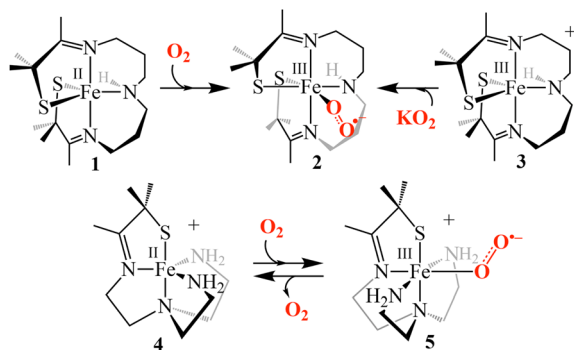
Scheme 1 Pathways for the formation of [\text{Fe}^{\text{III}}(\text{S}_2\text{Me}_2\text{N}_3(\text{Pr,Pr}))(\text{O}_2)] (2) (top), and reversible dioxygen binding to [\text{Fe}^{\text{II}}(\text{S}^{\text{Me}_2}\text{N}_4(\text{tren}))]^+ (4) to form a putative superoxo intermediate [\text{Fe}^{\text{III}}(\text{S}^{\text{Me}_2}\text{N}_4(\text{tren}))(\text{O}_2)]^+ (5) (bottom).
