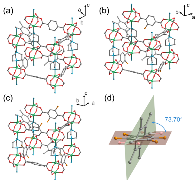
Fig. 1 Expanded cubic-like structure of (a) DMOF-0F , (b) DMOF-1F , and (c) DMOF-2F , in which only one orientation of the disordered xFBTC ligand is shown. (d) Disorder of 1FBD and 2FBD in DMOF-1F . Hydrogen atoms are omitted for clarity. Colour code: C: grey; F: orange; N: blue; O: red; Zn: green.
