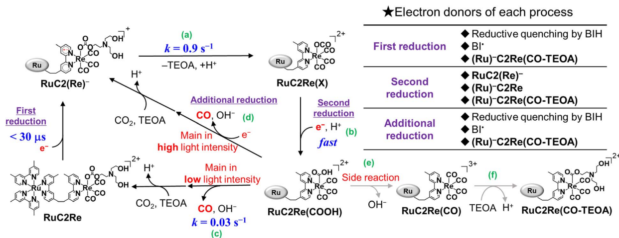
Scheme 5 Full reaction mechanism of photocatalytic \text{CO}_2 reduction by using \text{RuC}_2\text{Re} and BIH.
