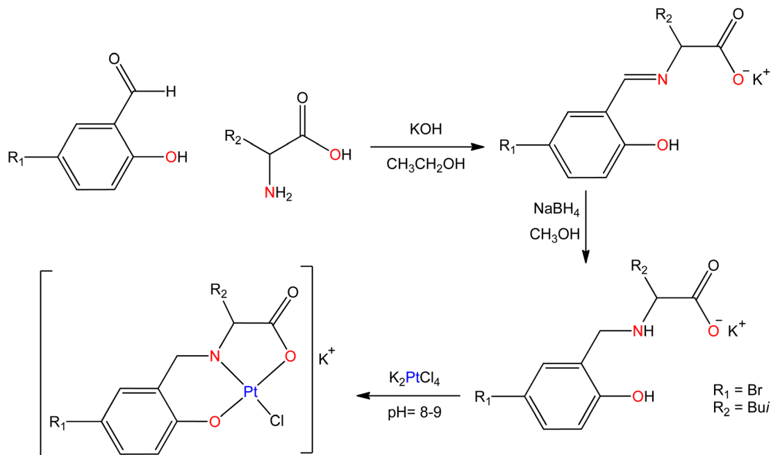
Fig. 21 Synthetic pathway of water-soluble Pt(II) complexes of amino acid SB.
