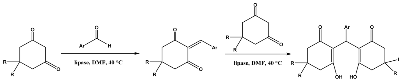
Fig. 20 Lipase-catalyzed Knoevenagel–Michael cascade reactions of aromatic aldehydes and 1,3-cyclodiketones.
