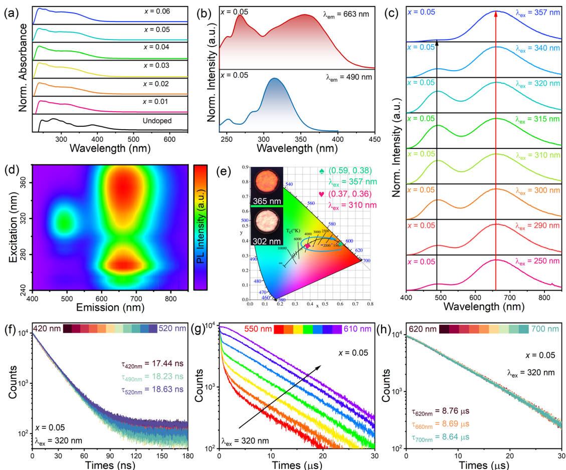
Fig. 2 (a) Absorption spectra of the (\text{TMA})_2\text{HfCl}_6:\text{xSb}^{3+} ( \text{x} = 0-0.06 ). (b) PL excitation (PLE) of 663 and 490 nm emission in (\text{TMA})_2\text{HfCl}_6:0.05 \text{Sb}^{3+} crystals. (c) PL spectra of (\text{TMA})_2\text{HfCl}_6:\text{Sb}^{3+} under different excitation wavelengths varying from 250 to 357 nm. (d) Contour plot of the excitation-dependent photoluminescence of the (\text{TMA})_2\text{HfCl}_6:0.05 \text{Sb}^{3+} crystals. (e) The corresponding CIE color coordinates of the (\text{TMA})_2\text{HfCl}_6:0.05 \text{Sb}^{3+} samples under different excitation wavelengths. (the inset are the photos of the as-prepared samples under different UV lamp). PL decay curves of (\text{TMA})_2\text{HfCl}_6:0.05 \text{Sb}^{3+} in emission wavelength range of (f) 420–450 nm, (g) 550–610 nm, and (h) 620–700 nm excited by 320 nm.
