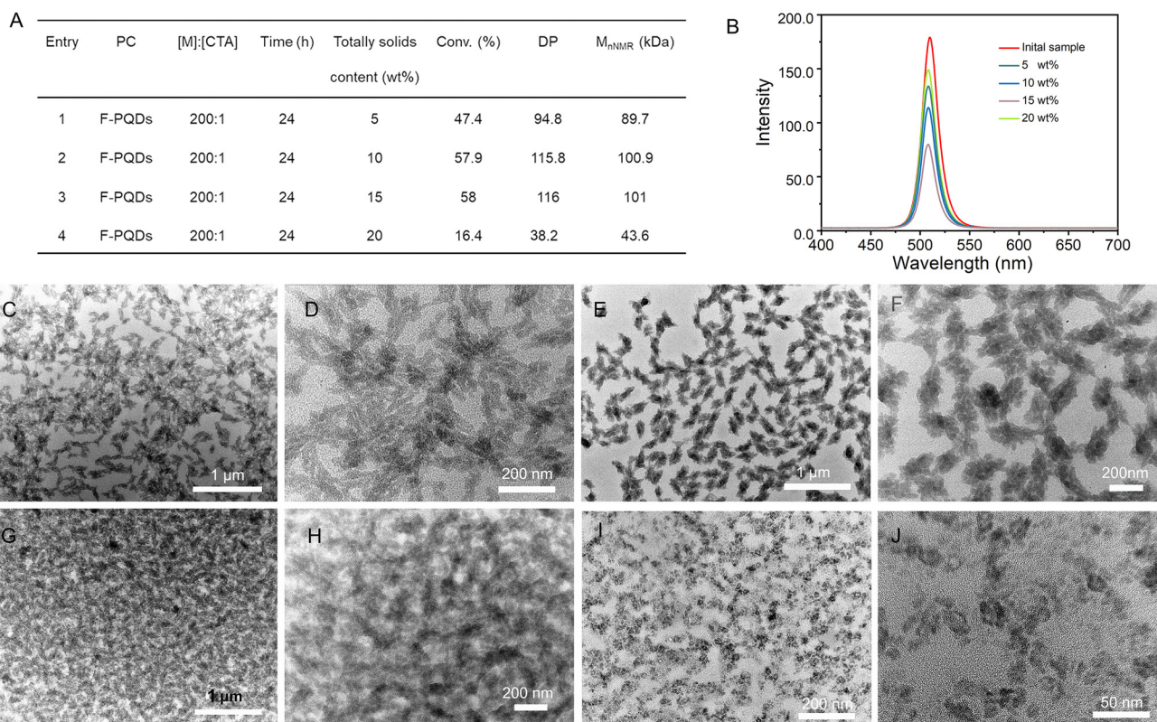
Fig. 2 (A) Characterization of POEGMA 78 - b -PFOEMA diblock copolymers synthesized with a different total solid content, (B) PL spectra (excited at 380 nm) of self-assembled POEGMA 78 - b -PFOEMA nanoparticles in toluene, and (C–J) TEM images of self-assembled POEGMA 78 - b -PFOEMA nanoparticles.
