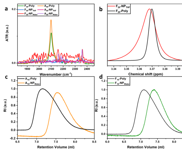
Fig. 1 (a) ATR-IR absorption spectra for F_{30} -poly, F_{30}\text{-NP}_{\text{THF/water}} , A_{30} -poly and A_{30}\text{-NP}_{\text{THF/water}} . (b) ^1\text{H-NMR} spectra in CDCl 3 of F_{20} -poly (black) and F_{20}\text{-NP}_{\text{THF}} (red). SEC curves in THF for (c) A_{10} -poly and A_{10}\text{-NP}_{\text{water}} and (d) F_{10} -poly and F_{10}\text{-NP}_{\text{water}} .
