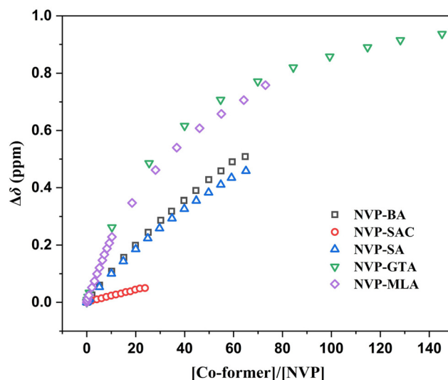
Fig. 2 ^1\text{H} NMR proton positions of NVP proton 1 with different co-formers as function of co-former concentration in acetone- d_6 .
