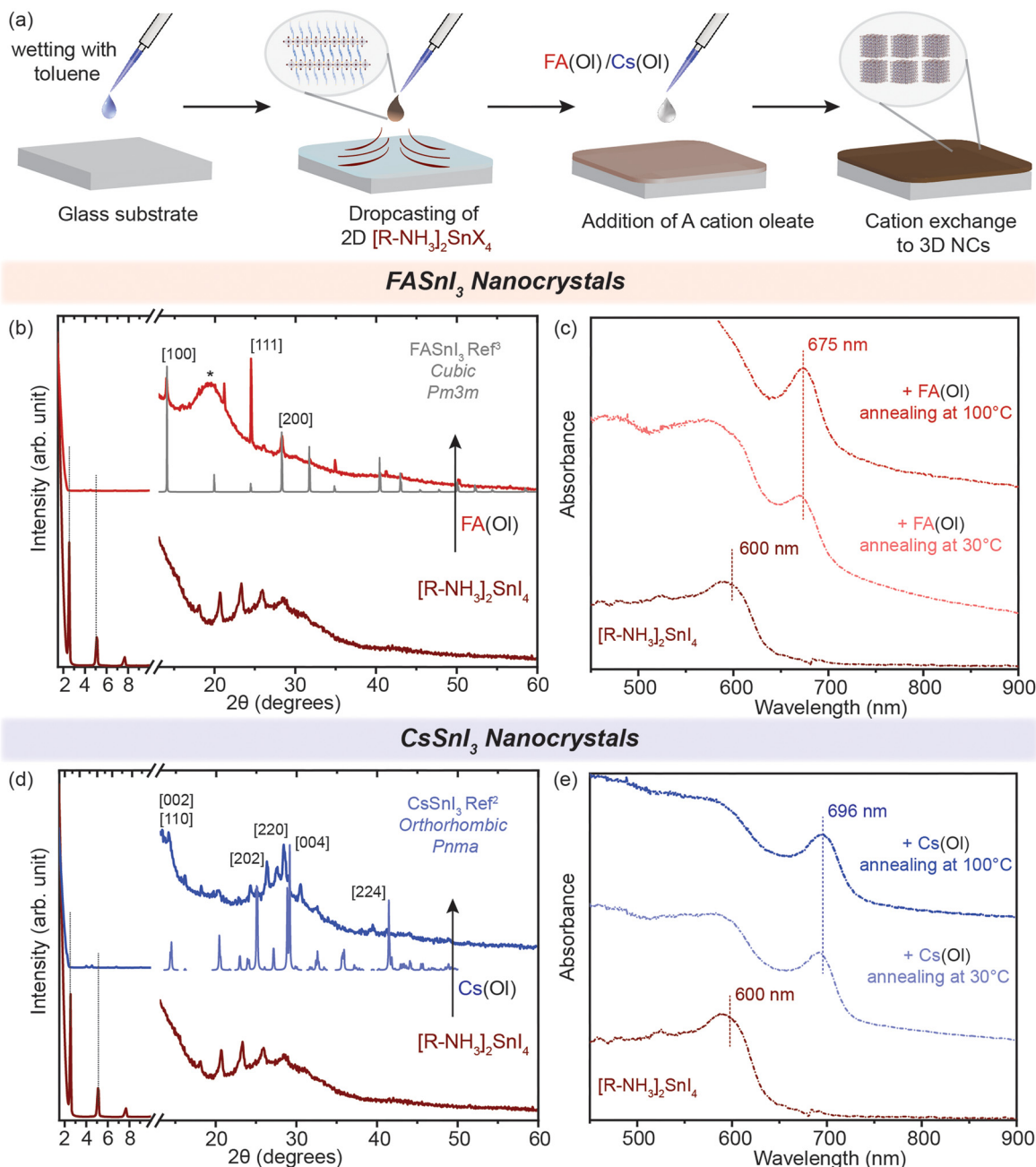
Fig. 4 Cation exchange in thin films. (a) Schematic of the methodology utilized to fabricate the thin films. (b and d) Powder XRD patterns of the converted 3D FASn 3 (red) and CsSn 3 (blue) NC thin film from the 2D [R-NH 3 ] 2 SnI 4 RP perovskite, respectively. (c and e) UV-visible spectroscopy of the formation of the 3D FASn 3 (red) and CsSn 3 (blue) nanocrystal thin film from the 2D [R-NH 3 ] 2 SnI 4 RP structure annealed at 30 °C and 100 °C for 1 h. * marks the peak arising from the glass substrate in the dome XRD sample holder. The XRD references are adapted from ref. 3 for FASn 3 (cubic, Pm\bar{3}m ) and ref. 2 for CsSn 3 (orthorhombic, Pnma ).
