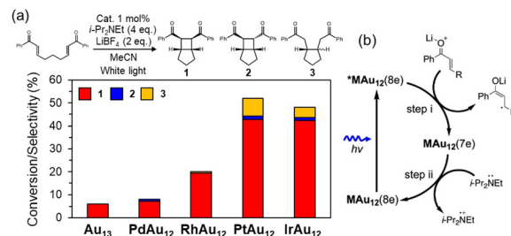
Fig. 6 (a) Comparison of the photoredox catalytic properties of \text{MAu}_{12}(\text{dppe})_5\text{Cl}_2 (M = Au, Pd, Pt, Rh, or Ir). (b) Proposed reaction mechanism for \text{MAu}_{12} , a so-called oxidative quenching cycle. Reproduced from ref. 58 with permission from Wiley-VCH, Copyright 2023.
