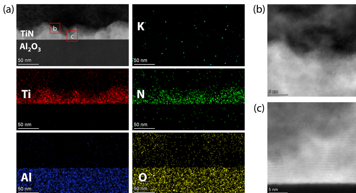
Fig. 7 (a) HAADF-STEM image of TiN films on \text{Al}_2\text{O}_3 substrates immersed in KOH for 10 days, combined with the EDX mapping of K, Ti, N, Al, and O elements. (b) Enlargement of the top area as depicted in (a). (c) Atomic-resolution image of TiN films at the interface of the film and the substrate as depicted in (a).
