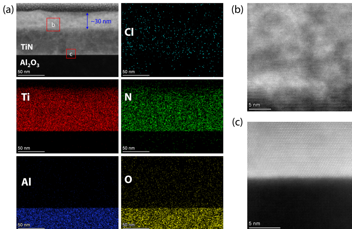
Fig. 6 (a) HAADF-STEM image of TiN films on \text{Al}_2\text{O}_3 substrates immersed in HCl for 7 days, combined with the EDX mapping of Cl, Ti, N, Al, and O. (b) Enlargement of the brighter area as depicted in (a). (c) Atomic-resolution image of the TiN film at the interface of the film and the substrate as depicted in (a).
