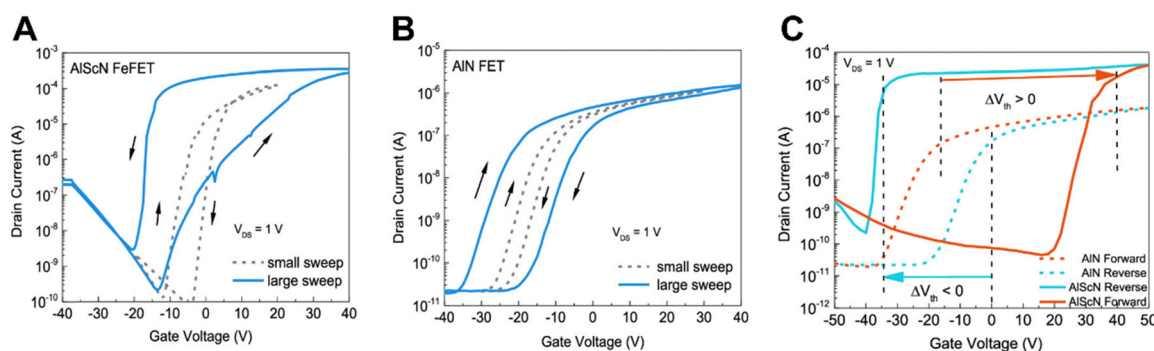
Fig. 3 Comparison of the ScAlN/MoS 2 FE-FET with the reference AlN/MoS 2 FET. 43 (A), (B) Transport characteristics of representative ScAlN/MoS 2 FE-FET and AlN/MoS 2 FET in semilogarithmic scale at room temperature with larger gate voltage sweep range (solid blue line) and smaller gate voltage sweep range (gray dashed line). Film thickness is 100 nm and the channel length is about 3.75 \mu\text{m} . (C) Comparison of the transfer characteristics of ScAlN and AlN dielectric molybdenum disulfide FET during forward and reverse scans in the \pm 50 V range.
