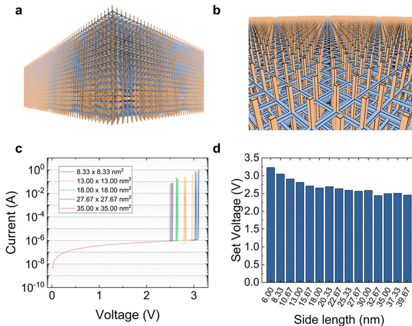
Fig. 5 (a) Resistance network corresponding to a great area (100 nm \times 100 nm) device. (b) Resistance network corresponding to a great area (100 nm \times 100 nm) device (zoomed-in view). (c) Several simulated set I - V curves for different device areas (the current values are scaled with respect to the lowest area shown in the plot, i.e. (8.33 nm \times 8.33 nm)). (d) Set voltage versus device side length (assuming a device square area obtained as (side length) 2 ).
