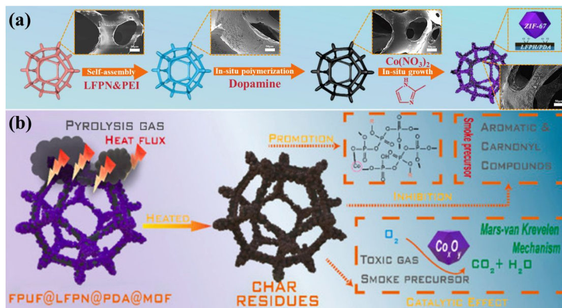
Fig. 10 (a) Preparation process and (b) flame retardant mechanism of FPUF@LFPN@PDA@MOF.
