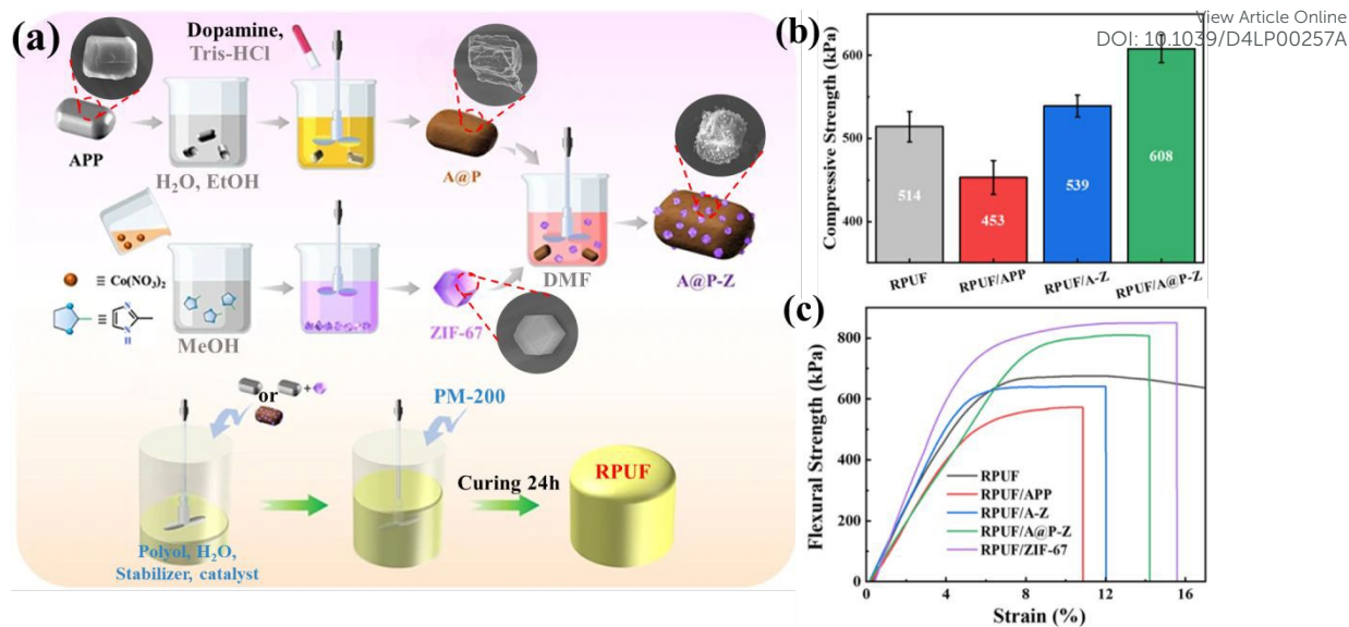
Fig. 9 (a) Flow chart for the preparation of A@P-Z and RPUF composites; (b) 10 % compressive strength and (c) flexural strength of RPUF and its composites. Reproduced with permission from ref. 86, copyright reserved Wiley 2018.
