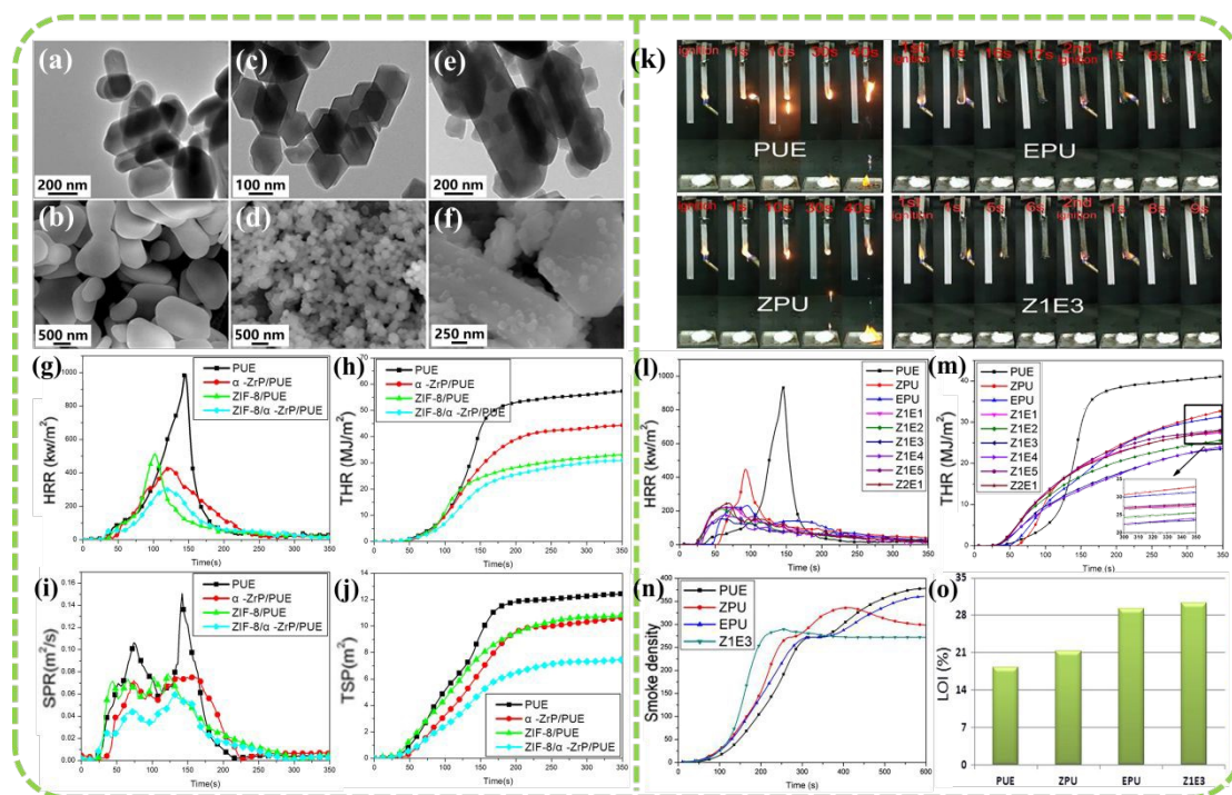
Fig. 3 TEM and SEM images of (a, b) \alpha -ZrP, (c, d) ZIF-8, and (e, f) ZIF-8/ \alpha -ZrP; (g) HRR, (h) THR, (i) SPR and (j) TSP curves. Reproduced with permission from ref. 46, copyright reserved Wiley 2018. (k) UL-94 vertical burning test; (l) HRR, (m) THR, (n) smoke density, and (o) LOI curves for pure PUE and PUE composites ( Z_xE_y denotes the ZIF-8 to EG ratio of x:y ). Reproduced with permission from ref. 47, copyright reserved Wiley 2019.
