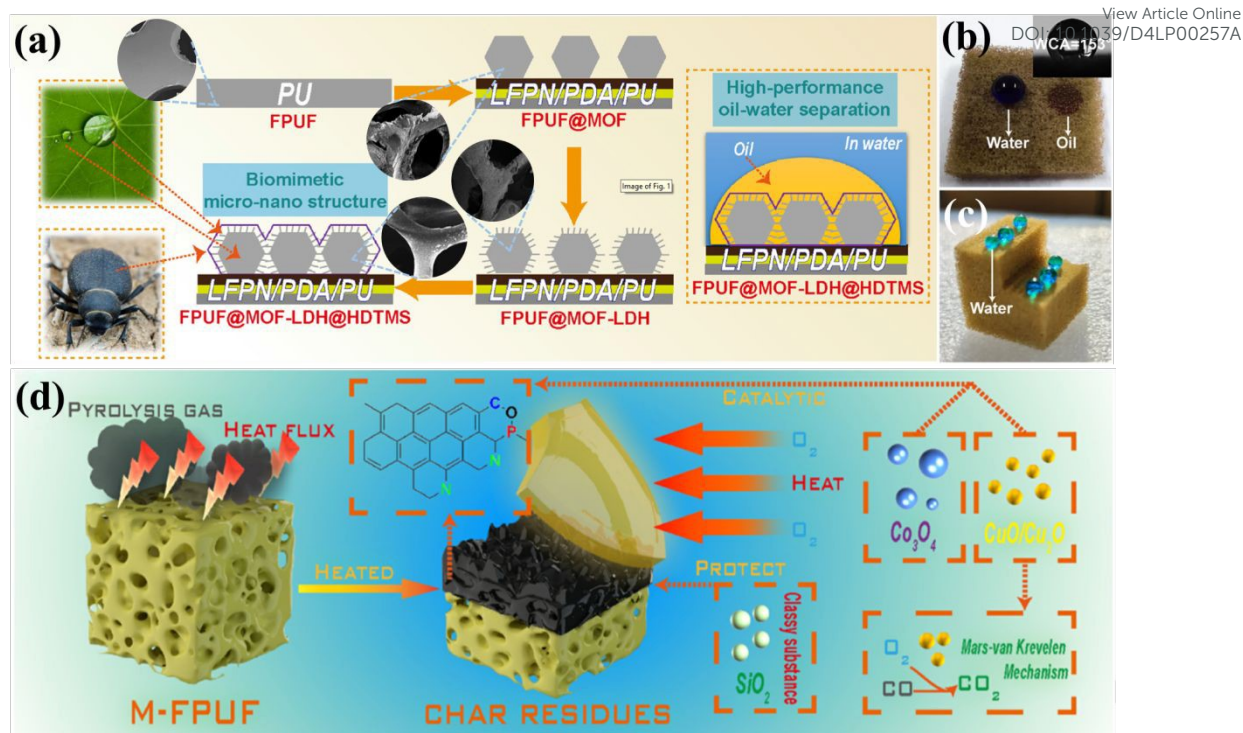
Fig. 13 (a) Schematic of FPUF@MOF-LDH@HDTMS bionic structure and oil-water separation mechanism; (b, c) wettability of FPUF@MOF-LDH@HDTMS; (d) flame retardant mechanism of FPUF composite. Reproduced with permission from ref. 94, copyright reserved Elsevier 2023.
