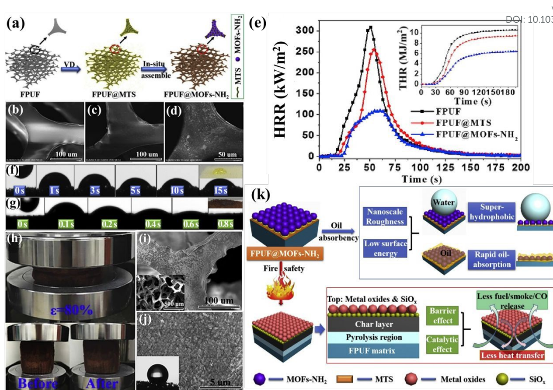
Fig. 11 (a) Schematic diagram of FPUF@MOFs-NH 2 sponge preparation process; SME images of pure (b) FPUF, (c) FPUF@MTS, and (d) FPUF@MOFs-NH 2 ; (e) heat release curves of FPUF and its composites; absorption process of soybean oil by (f) pure FPUF and (g) FPUF composite sponge; (h) digital images of FPUF composite sponge compression test; (i, j) SEM images of FPUF composite sponge after 1000 compression tests at different magnifications; (k) Oil absorption and flame retardant mechanism diagram of FPUF composite sponge. Reproduced with permission from ref. 92, copyright reserved Elsevier 2019.
