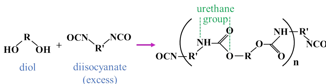
Fig. 1 Reaction scheme of preparing PU.
