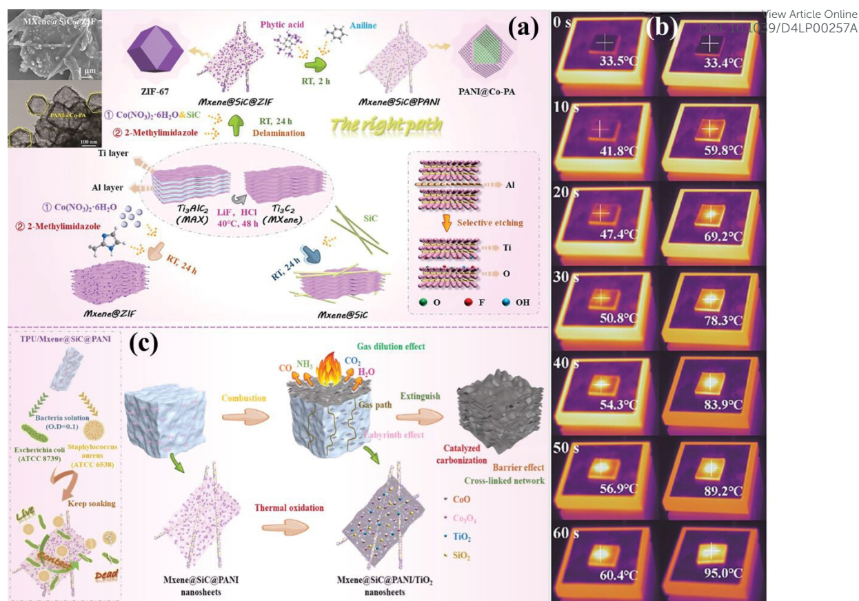
Fig. 7 (a) Schematic of the synthesis of MXene@SiC@PANI; (b) infrared thermography of TPU/MXene@SiC@PANI composites during heating; (c) antimicrobial process and flame-retardant mechanism of composite TPU. Reproduced with permission from ref. 73, copyright reserved Wiley 2024.
